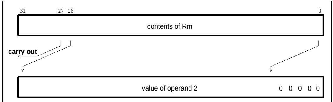
Figure 4-6: Logical shift left
