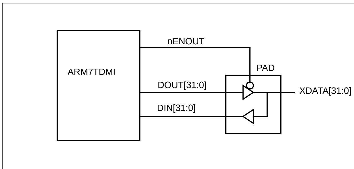
Figure 6-13: External connection of unidirectional busses
